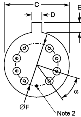
Variants 03, 04, 05 (9 leads)
