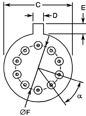
Variants 01, 02, 03 (10 leads)
