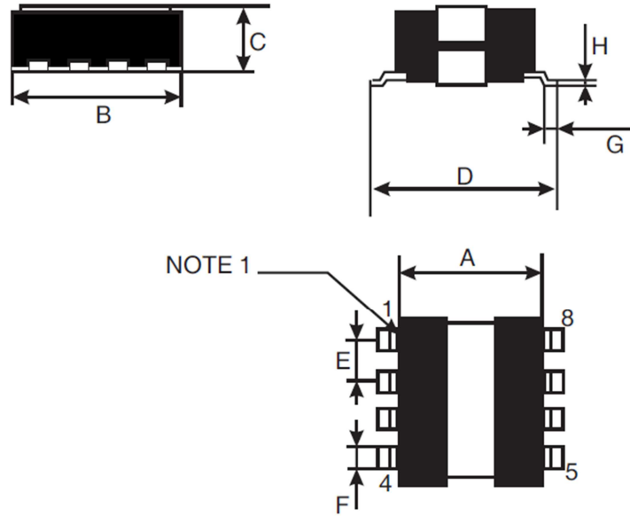
FIGURE 2 - PHYSICAL DIMENSIONS
