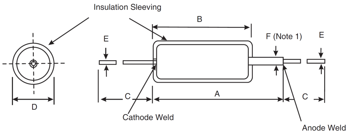
FIGURE 2 - PHYSICAL DIMENSIONS
