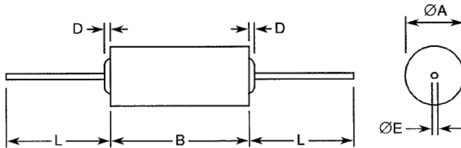
FIGURE 2 - PHYSICAL DIMENSIONS
