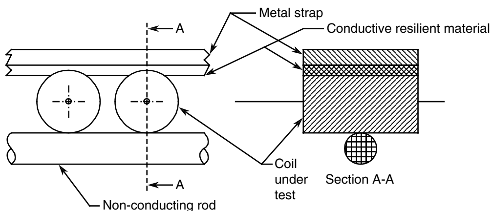
FIGURE 1 - COIL-CONTACTING ASSEMBLY FOR MOUNTING DURING POLARISATION
