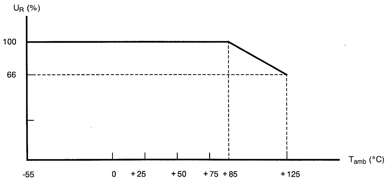
Rated Voltage versus Temperature
