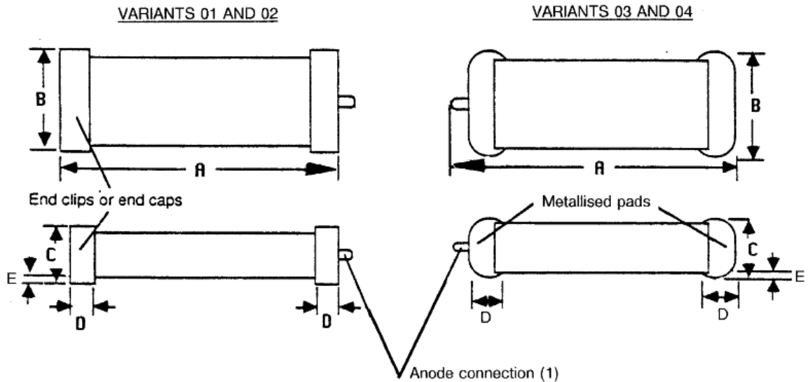
FIGURE 2 - PHYSICAL DIMENSIONS
