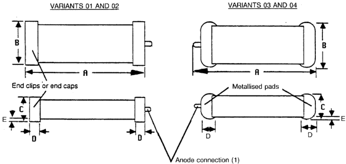
FIGURE 2 - PHYSICAL DIMENSIONS
