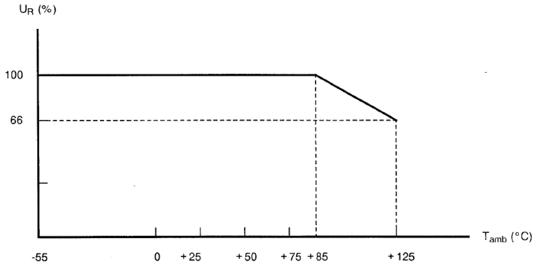
Rated Voltage versus Temperature
