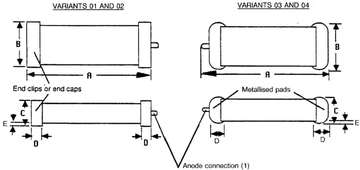
FIGURE 2 - PHYSICAL DIMENSIONS
