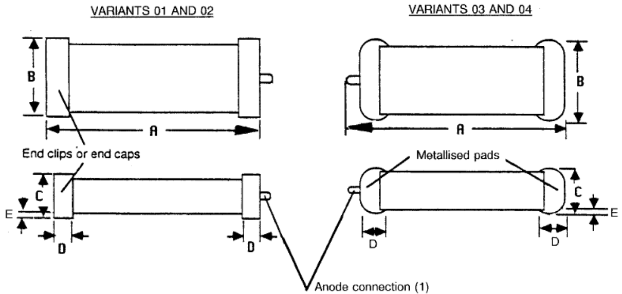
FIGURE 2 - PHYSICAL DIMENSIONS
