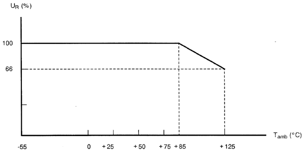
Rated Voltage versus Temperature
