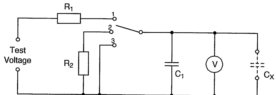
FIGURE I - VOLTAGE PROOF TEST CIRCUIT
