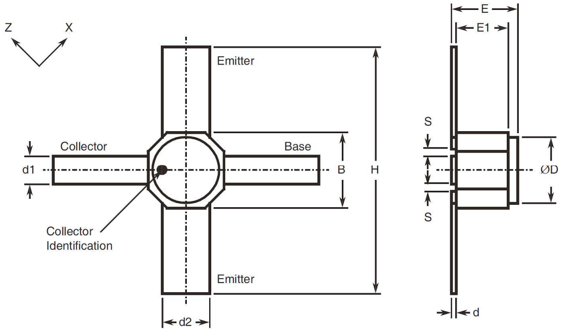
FIGURE 2 - PHYSICAL DIMENSIONS
