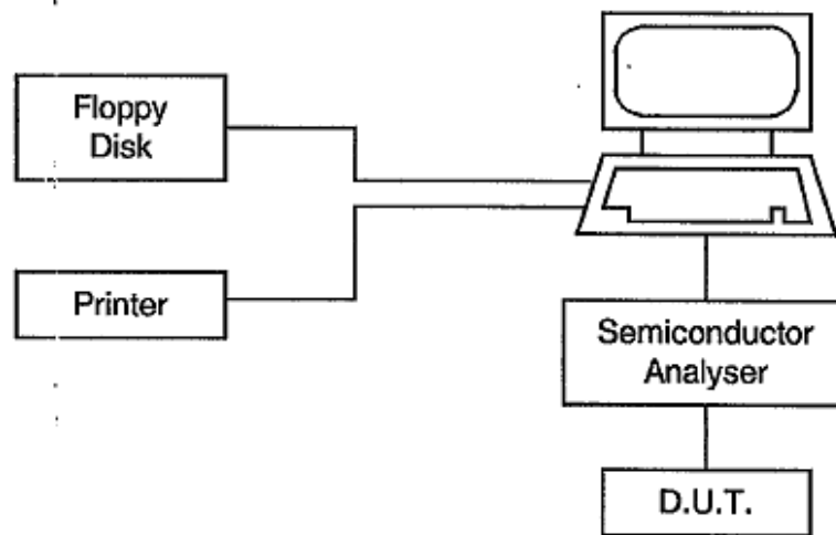
FIGURE 4(a) - TEST CIRCUIT FOR DC PARAMETERS
