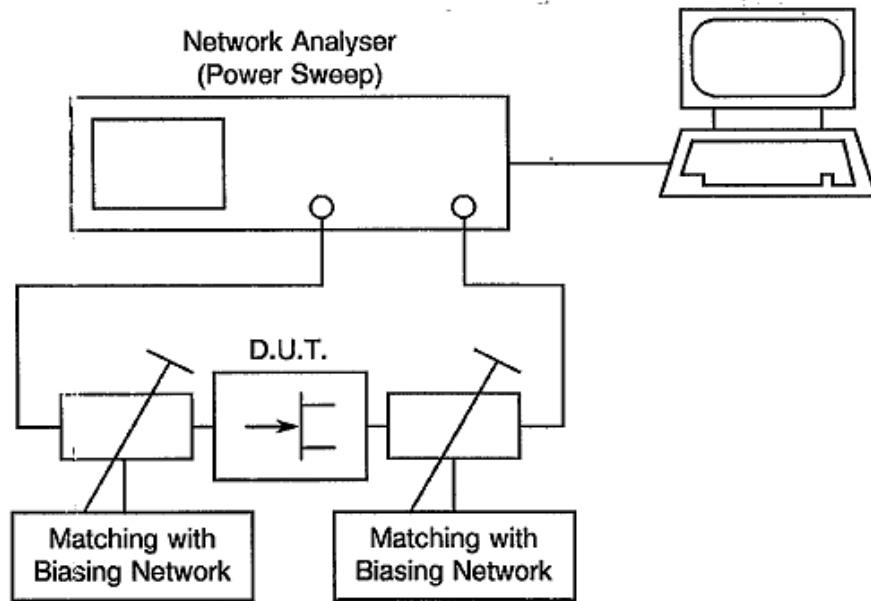
FIGURE 4(c) - TEST CIRCUIT FOR OUTPUT POWER MEASUREMENTS
