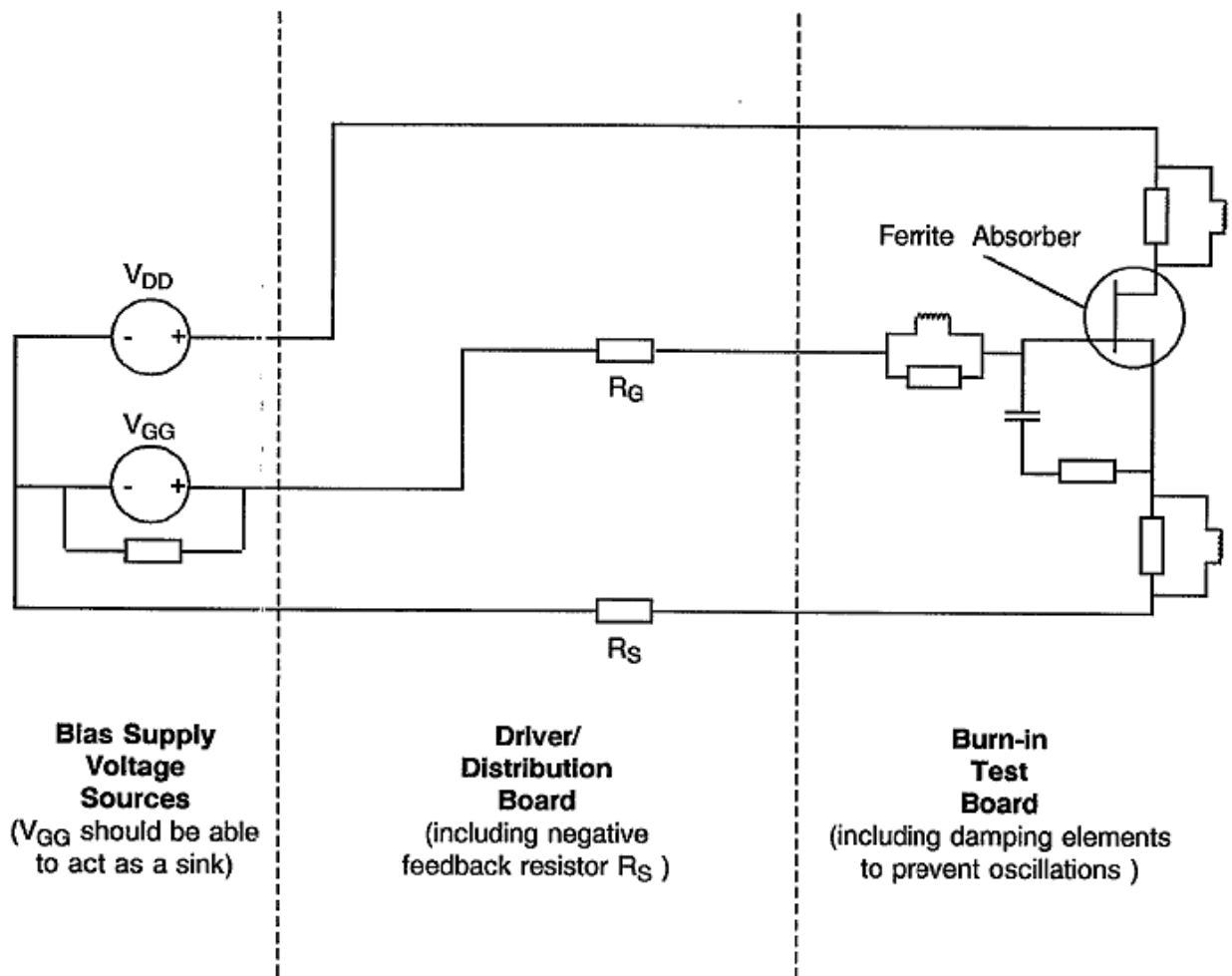
FIGURE 5 - ELECTRICAL CIRCUIT FOR BURN-IN
