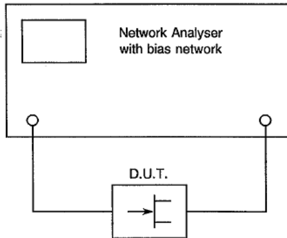
FIGURE 4(d) - TEST SET-UP FOR SCATTERING PARAMETER MEASUREMENTS
