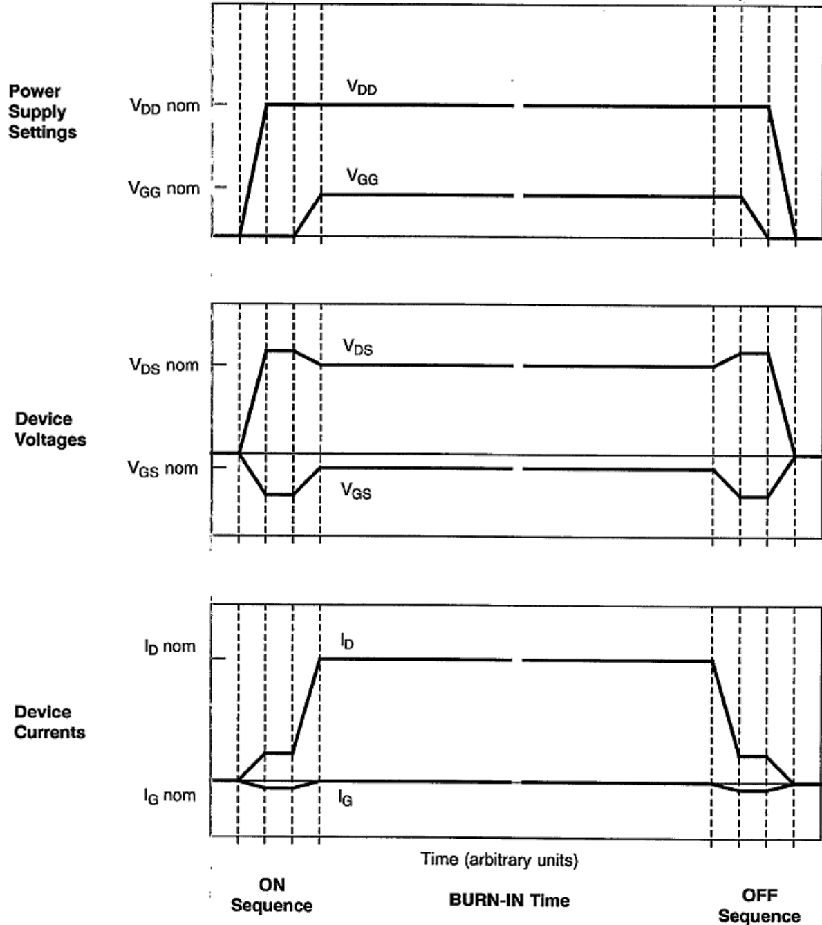
TIMING SEQUENCE FOR POWER BURN-IN ON/OFF BIASING
