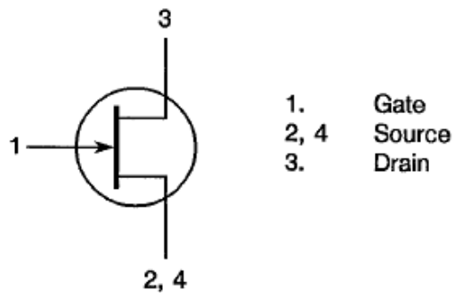
FIGURE 3 - FUNCTIONAL DIAGRAM
