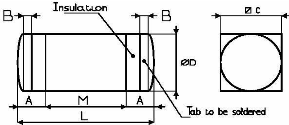
FIGURE 2 - PHYSICAL DIMENSIONS
