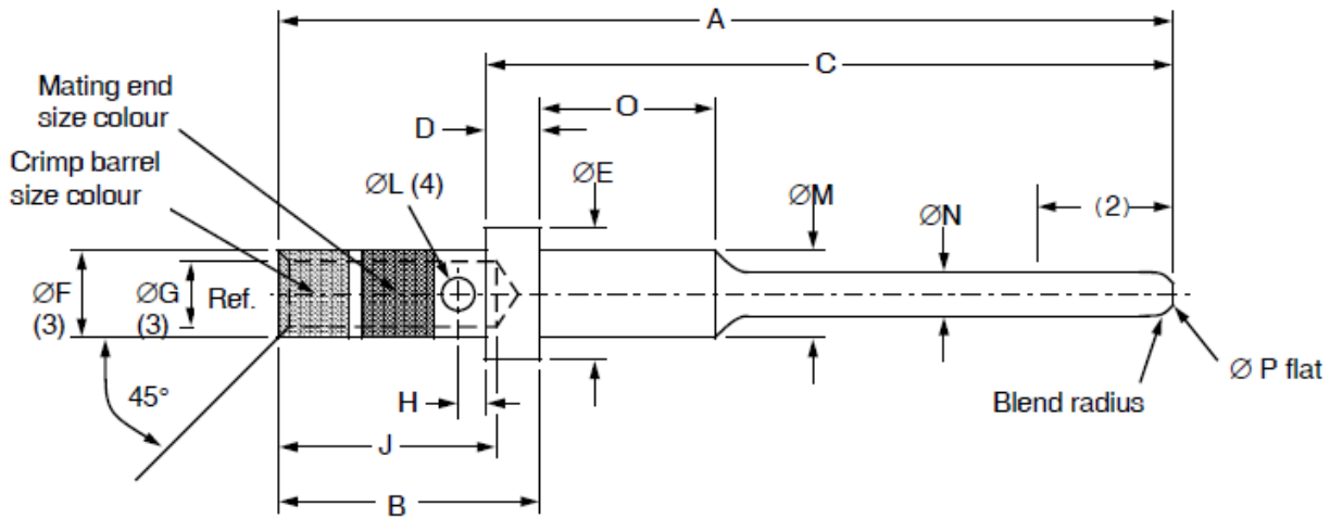
FIGURE 2 - PHYSICAL DIMENSIONS
