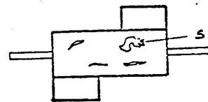
FIGURE 8 - CRACKS AND SCRATCHES IN PLATING
