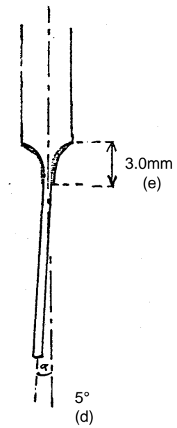
FIGURE 4 - TILTED LEAD
