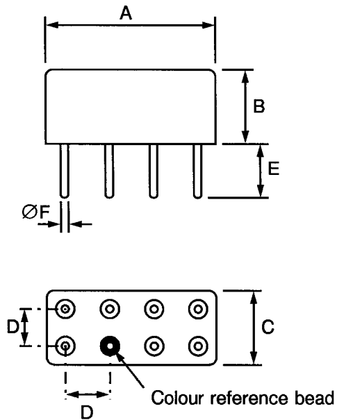
FIGURE 2(i) - VARIANT 09, RELAY WITH LONG PLUG-IN TERMINALS AND PLAIN CASE
