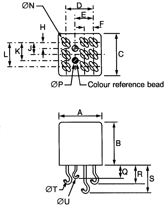
FIGURE 2(e) - VARIANT 06, RELAY WITH SOLDERABLE HOOK-END TERMINALS AND PLAIN CASE
