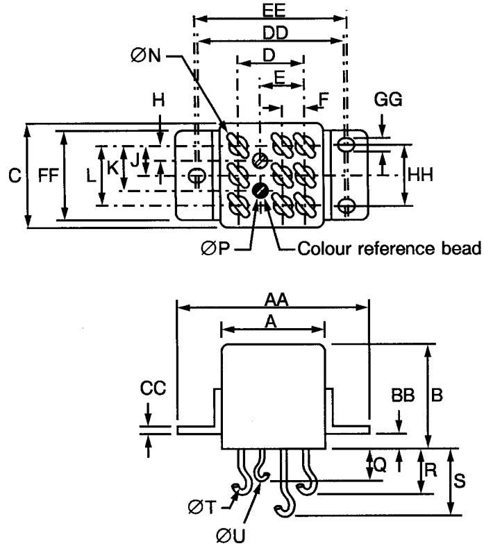
FIGURE 2(a) - VARIANT 02, RELAY WITH WITH SOLDERABLE HOOK-END TERMINALS AND HORIZONTAL FLANGE MOUNT
