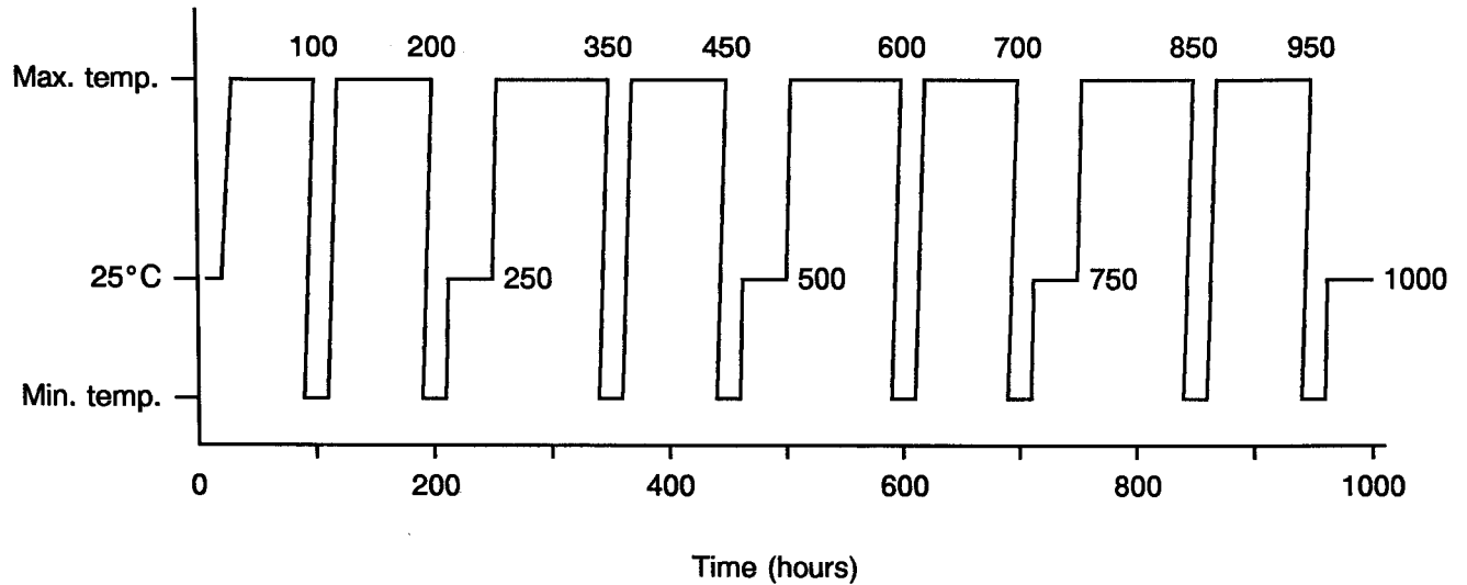
FIGURE II - AMBIENT TEMPERATURES
