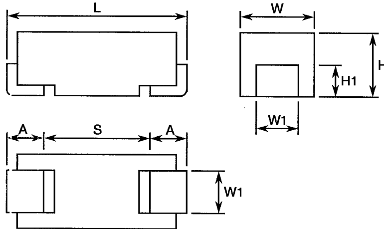
FIGURE 2 - PHYSICAL DIMENSIONS
