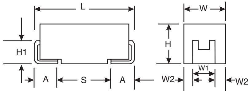
FIGURE 2 - PHYSICAL DIMENSIONS
