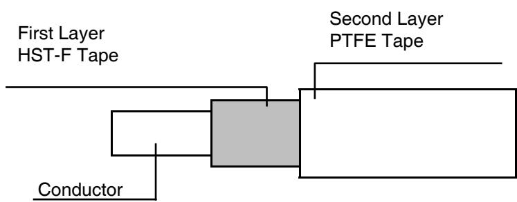
FIGURE 2(a) - FINISHED WIRES
