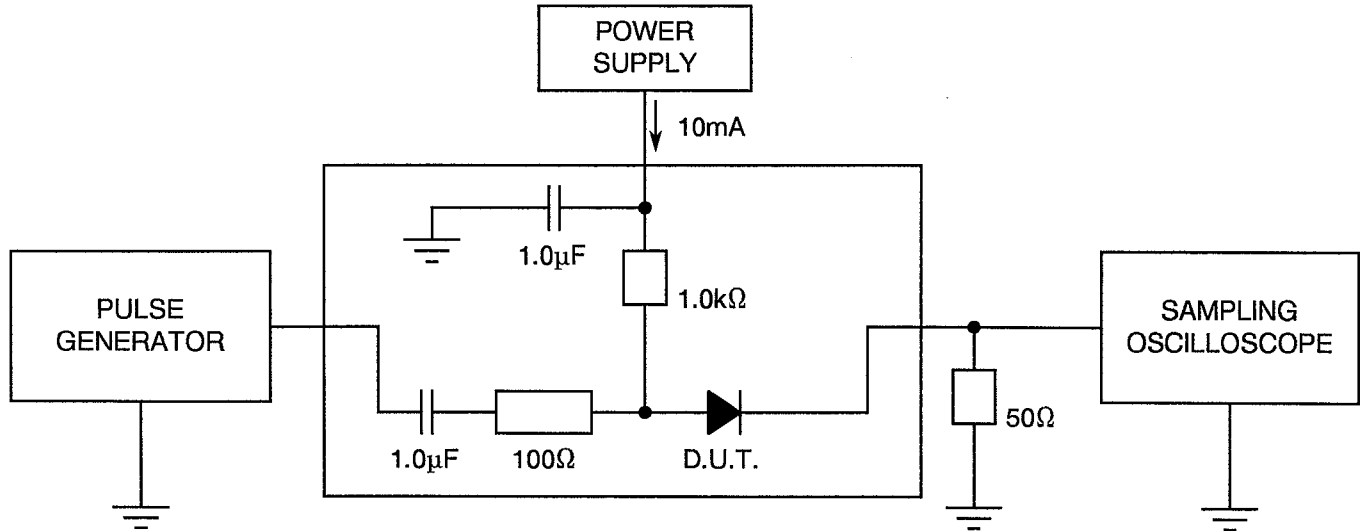
FIGURE 4 - TEST CIRCUIT FOR MINORITY CARRIER LIFETIME MEASUREMENT
