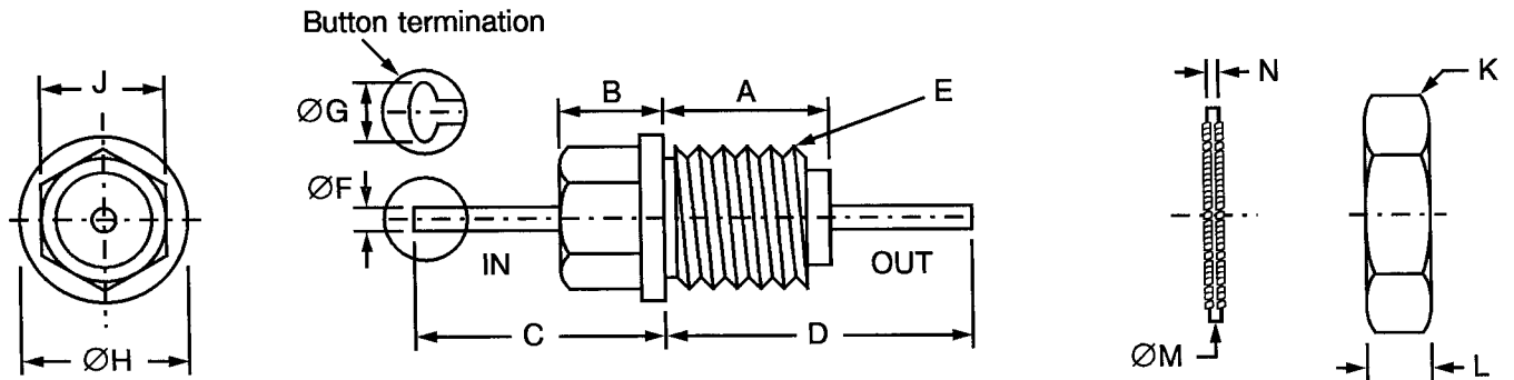
FIGURE 2 - PHYSICAL DIMENSIONS
