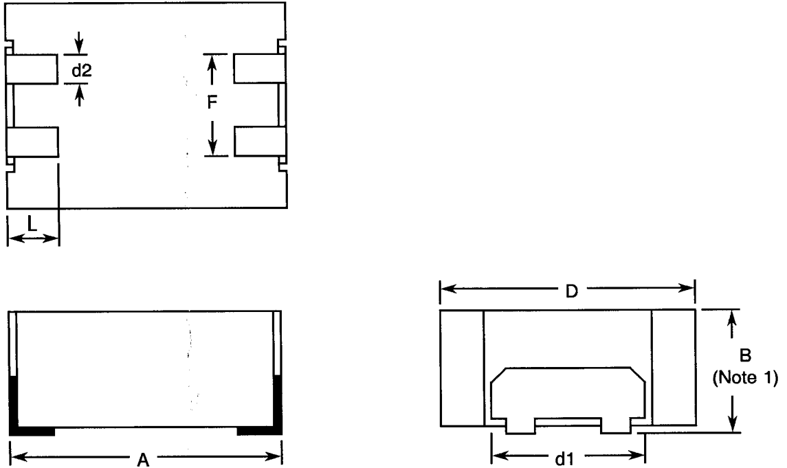
FIGURE 2 - PHYSICAL DIMENSIONS
