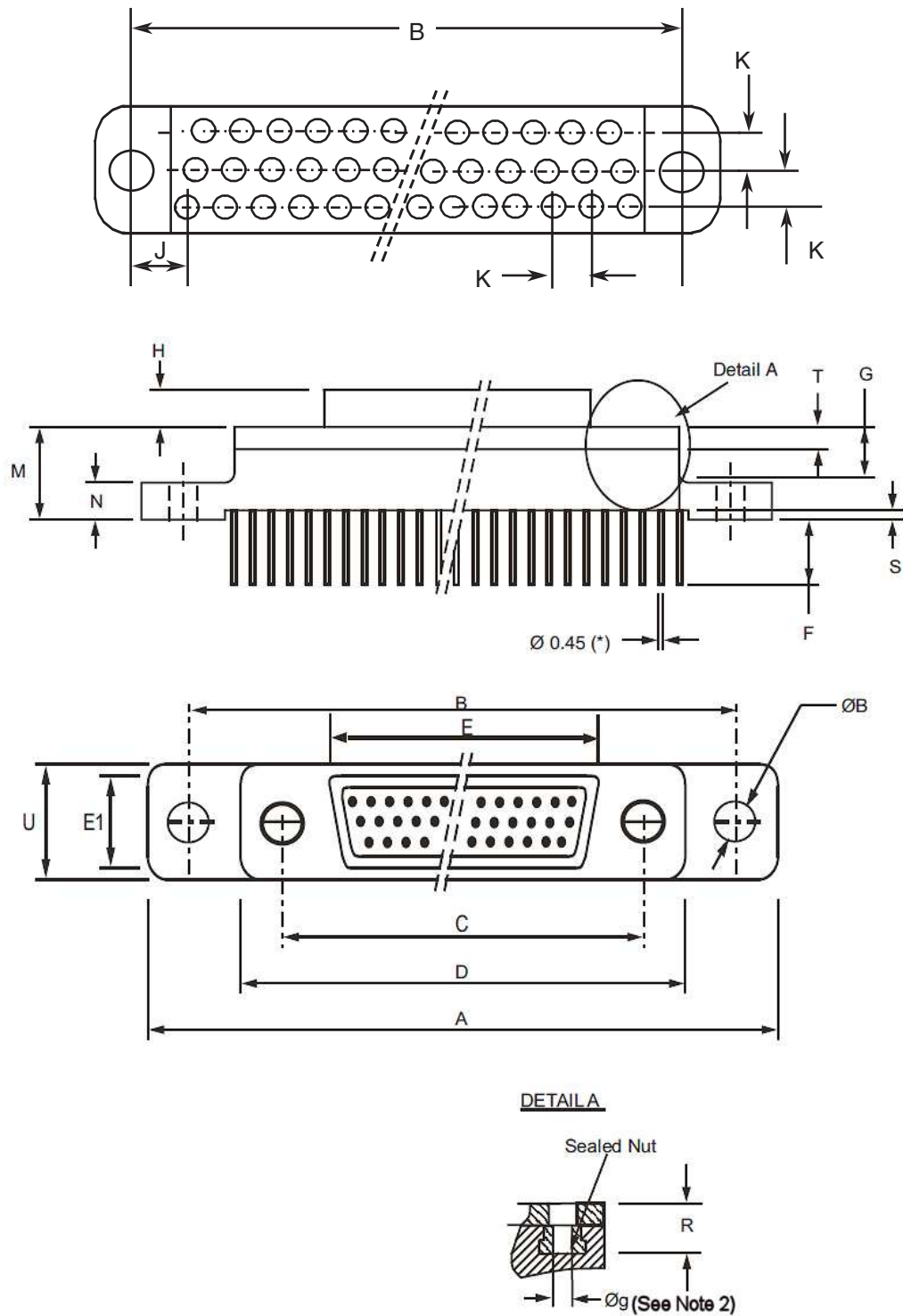
FIGURE 2.2I - CONNECTORS TYPE - FR139 PLUG MALE CONTACTS
