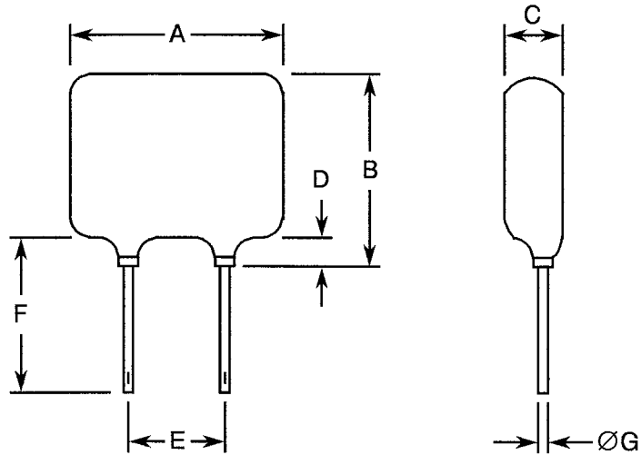
FIGURE 2 - PHYSICAL DIMENSIONS
