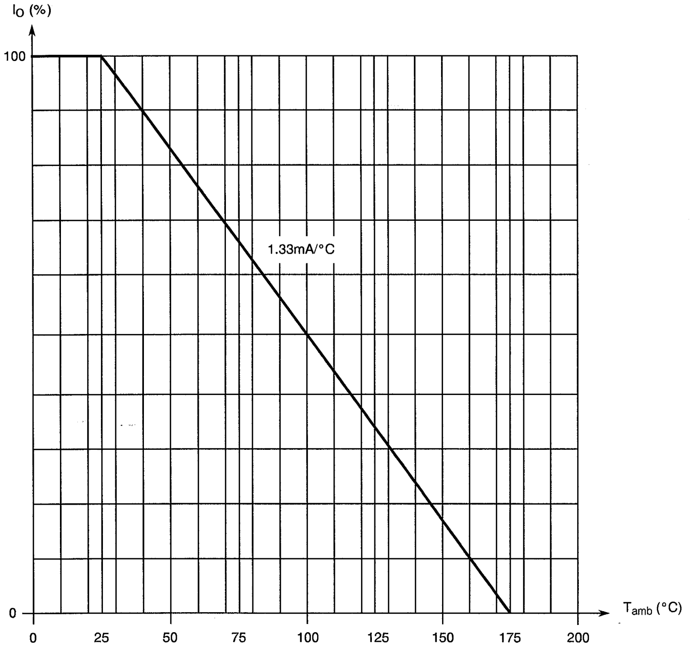
Average Output Rectified Current versus Temperature
