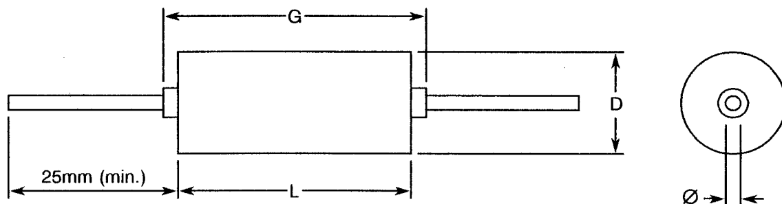
FIGURE 2 - PHYSICAL DIMENSIONS
