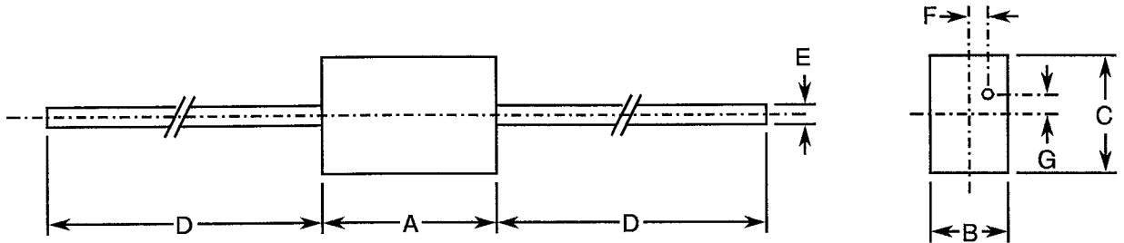
FIGURE 2 - PHYSICAL DIMENSIONS
