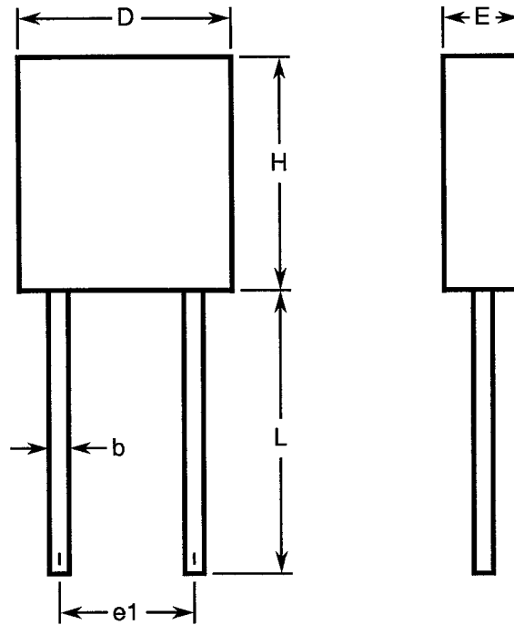
FIGURE 2 - PHYSICAL DIMENSIONS
