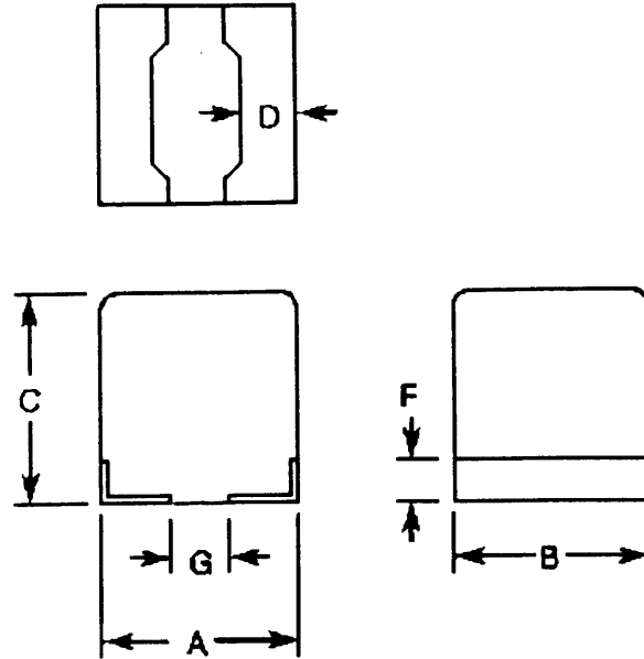
FIGURE 2 - PHYSICAL DIMENSIONS
