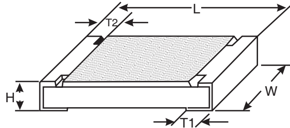
FIGURE 2 - PHYSICAL DIMENSIONS
