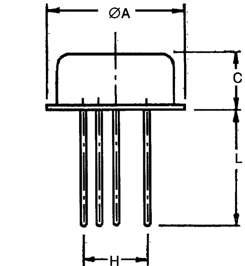
FIGURE 2 - PHYSICAL DIMENSIONS
