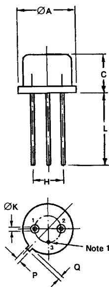
FIGURE 2(a) - 3-PIN PACKAGE Variant 01
