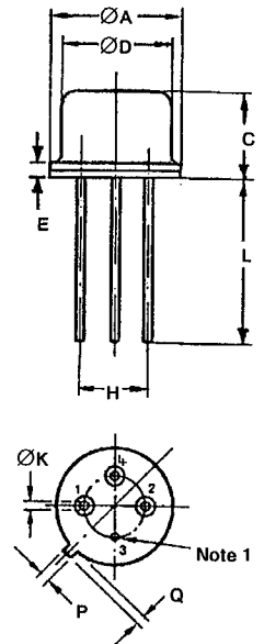
FIGURE 2(b) - 4-PIN PACKAGE Variant 02
