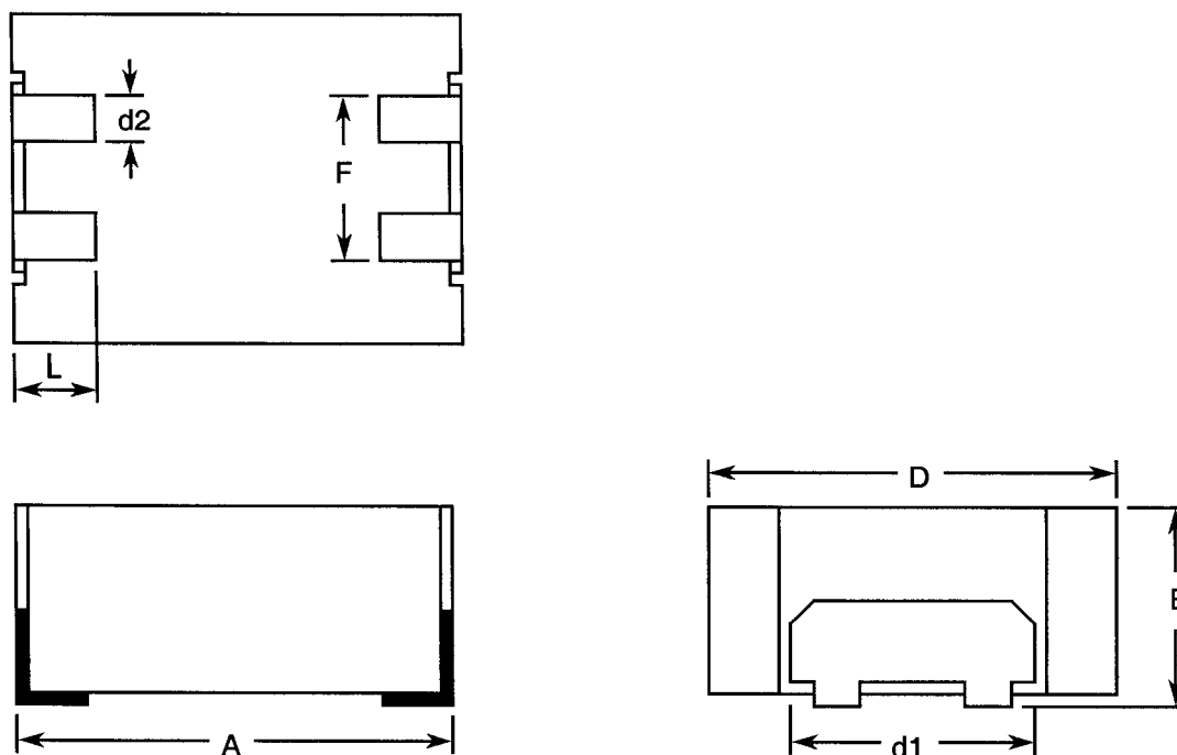
FIGURE 2 - PHYSICAL DIMENSIONS
