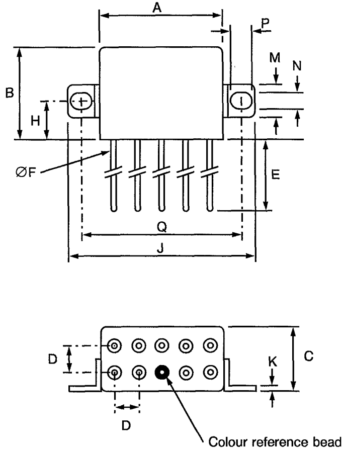
FIGURE 2(i) - VARIANT 10, RELAY WITH LEAD TERMINALS AND VERTICAL SHOULDER BRACKETS
