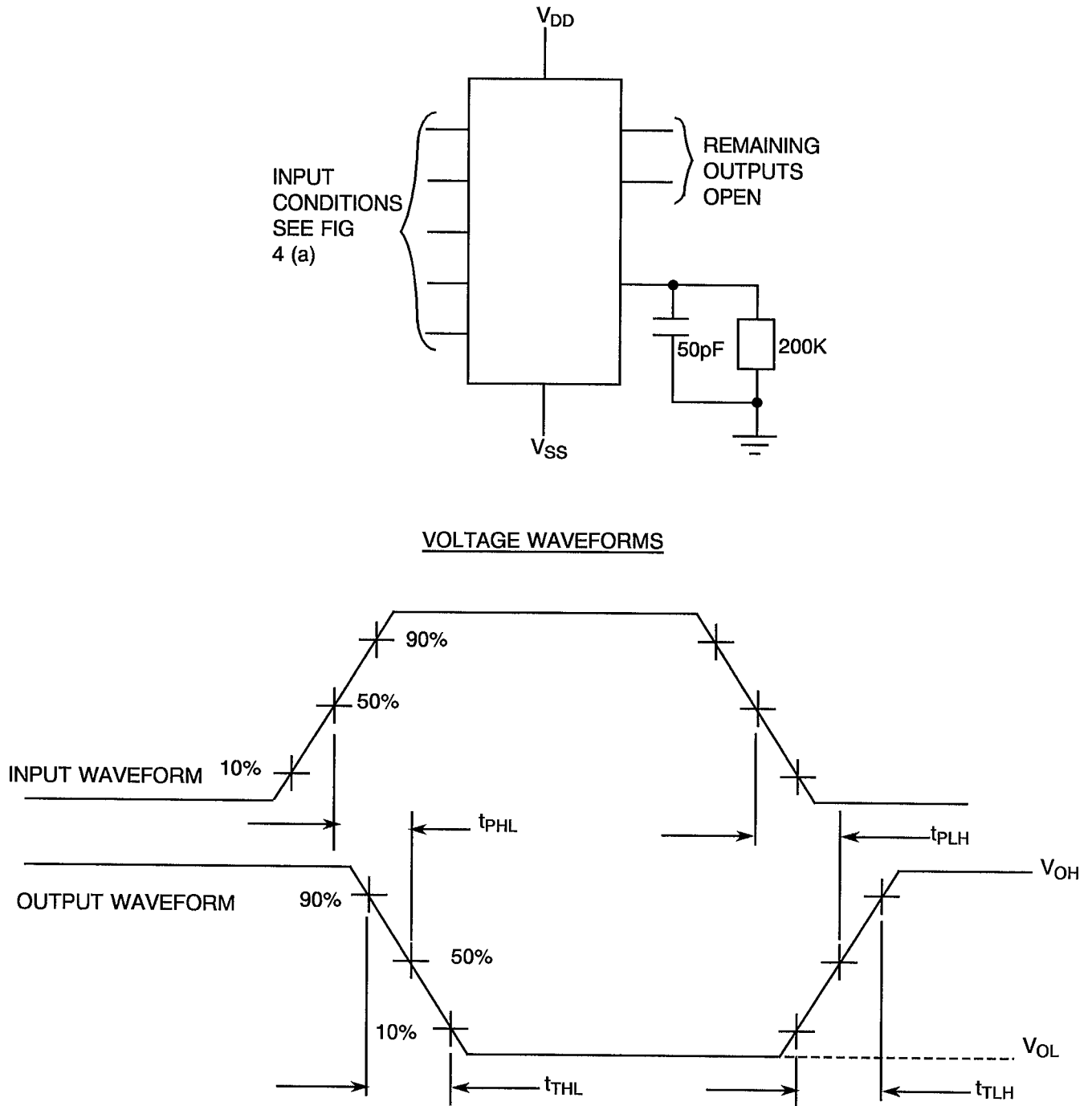
FIGURE 4(p) - PROPAGATION DELAY AND TRANSITION TIME
