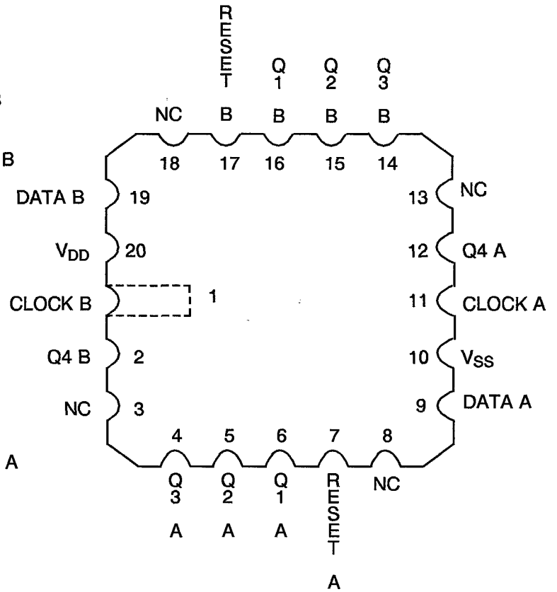
TOP VIEW
