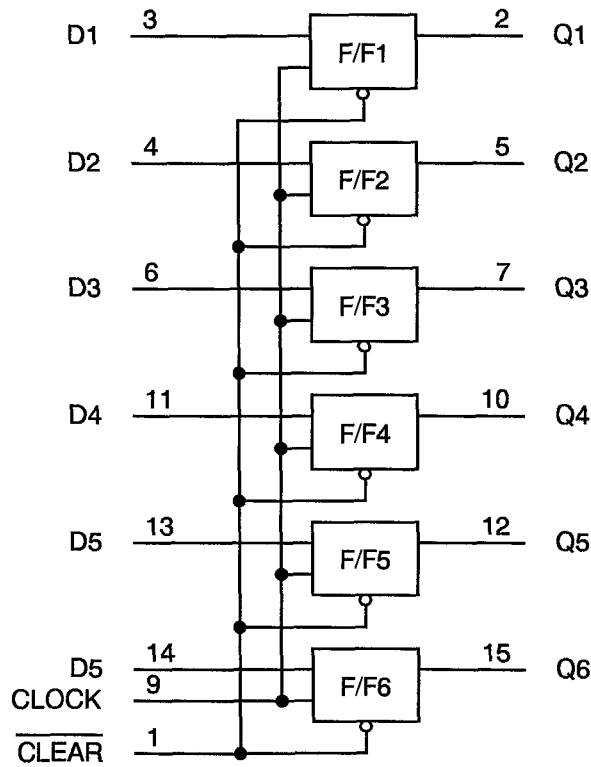
FIGURE 3(d) - FUNCTIONAL DIAGRAM
