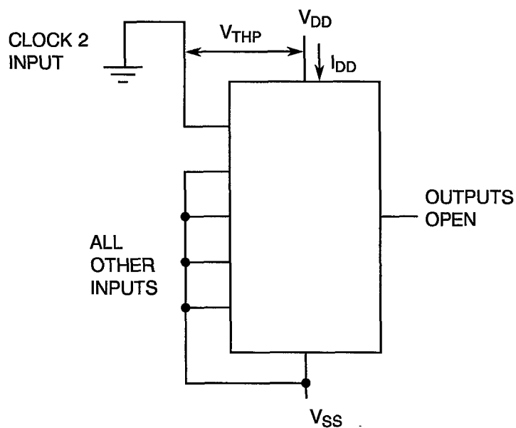
FIGURE 4(ii) - THRESHOLD VOLTAGE P-CHANNEL
