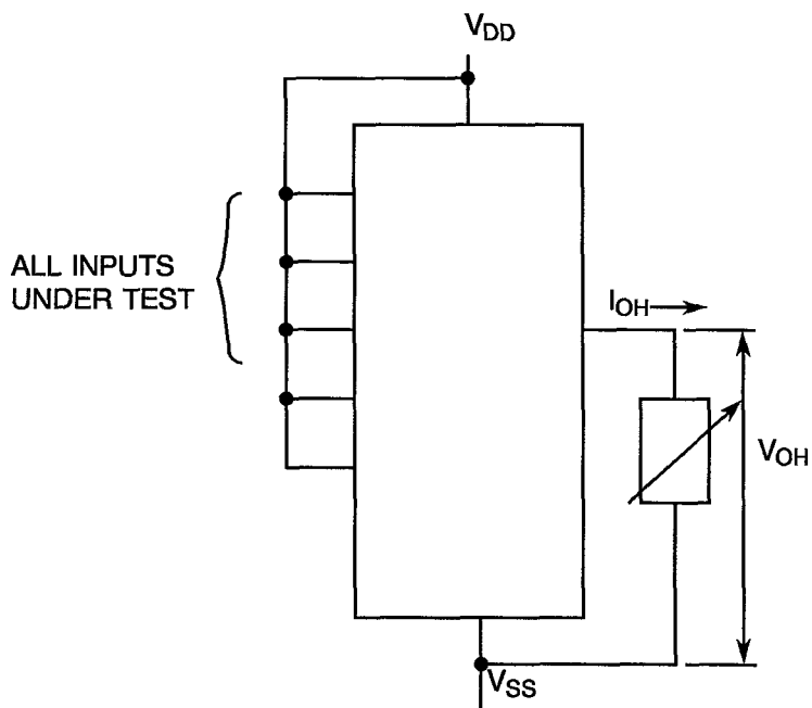
FIGURE 4(h) - HIGH LEVEL OUTPUT CURRENT
