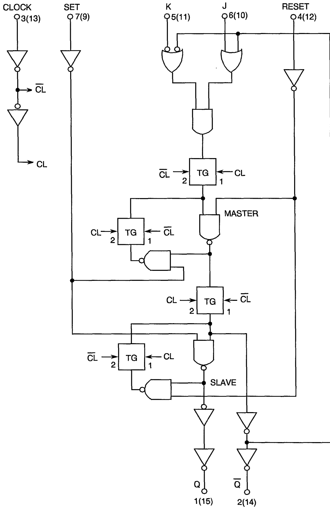
FIGURE 3(d) - FUNCTIONAL DIAGRAM (EACH FLIP-FLOP)
