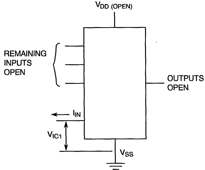
FIGURE 4(m) - INPUT CLAMP VOLTAGE ( V_{SS} )
