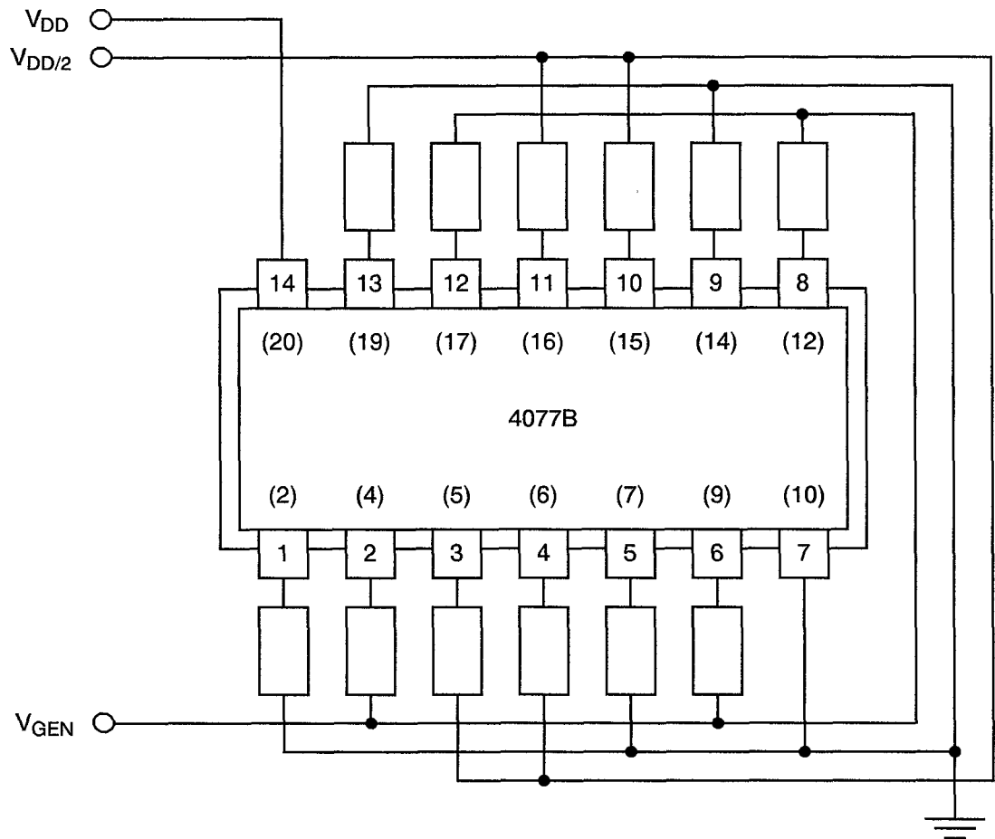
FIGURE 5(c) - ELECTRICAL CIRCUIT FOR BURN-IN DYNAMIC
