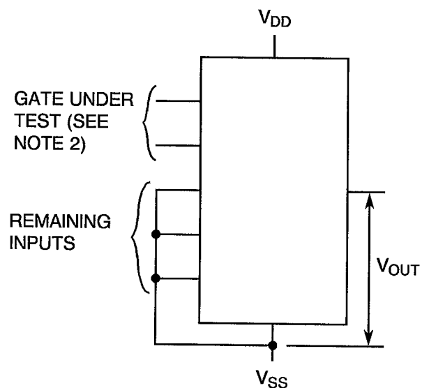
FIGURE 4(j) - HIGH LEVEL INPUT VOLTAGE
