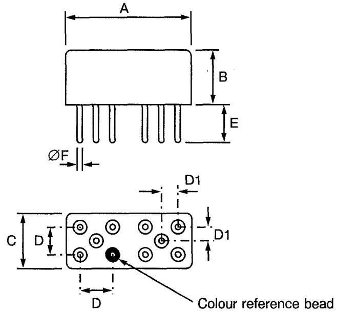
FIGURE 2(a) - VARIANT 01, RELAY WITH PLUG-IN TERMINALS AND PLAIN CASE
