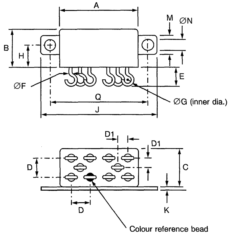
FIGURE 2(c) - VARIANT 03, RELAY WITH SOLDERABLE, HOOK-END TERMINALS AND VERTICAL SHOULDER BRACKETS
