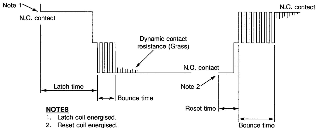
FIGURE I - TYPICAL OSCILLOSCOPE FIGURE OF LATCH, RESET AND CONTACT BOUNCE TIMES
