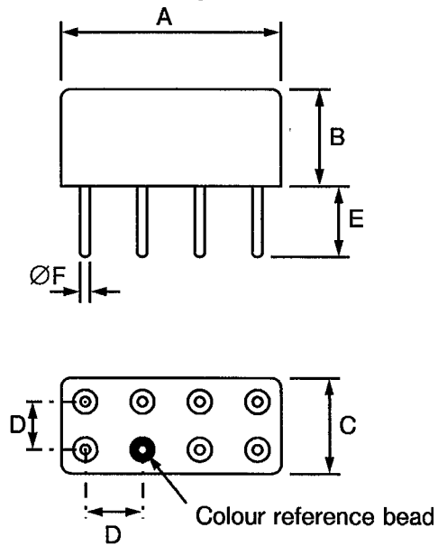
FIGURE 2(a) - VARIANT 01, RELAY WITH PLUG-IN TERMINALS AND PLAIN CASE
