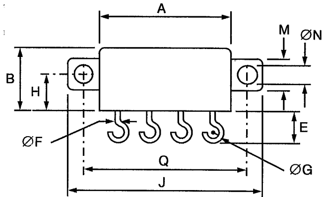
FIGURE 2(c) - VARIANT 03, RELAY WITH SOLDERABLE HOOK-END TERMINALS AND VERTICAL SHOULDER BRACKETS
