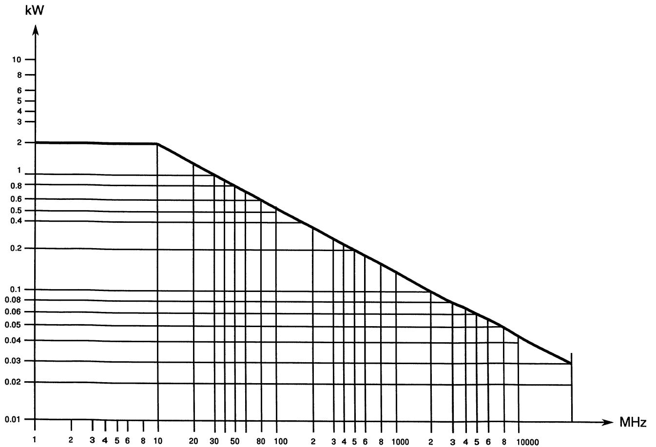
FIGURE 1(b) - POWER VERSUS FREQUENCY
