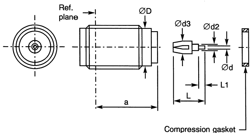
VARIANT 63 - HERMETIC BULKHEAD RECEPTACLE
