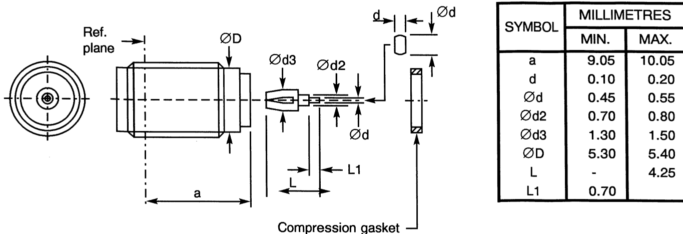
VARIANT 64 - HERMETIC BULKHEAD RECEPTACLE
